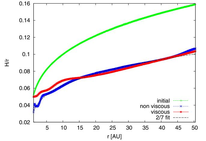
Fig. 4. Aspect ratio H/r of the stellar irradiated outer disc calculated using mid-plane values for discs with constant opacity \kappa = 1 \text{ cm}^2/\text{g} and constant viscosity. Starting from a flared disc profile the discs are evolved until they reach thermal equilibrium. These simulations differ from the ones presented in Fig. 2 only by the opening angle and radial extent of the disc.
